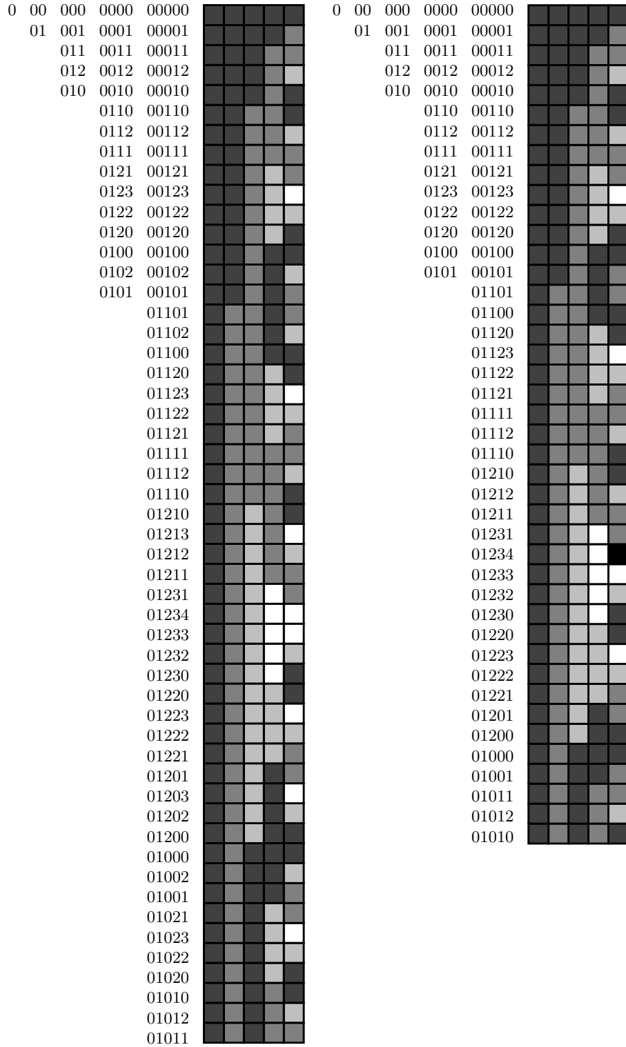
Figure 3: Gray codes obtained from our max-right algorithm: start from 0^n then greedily maximize the rightmost possible digit.
